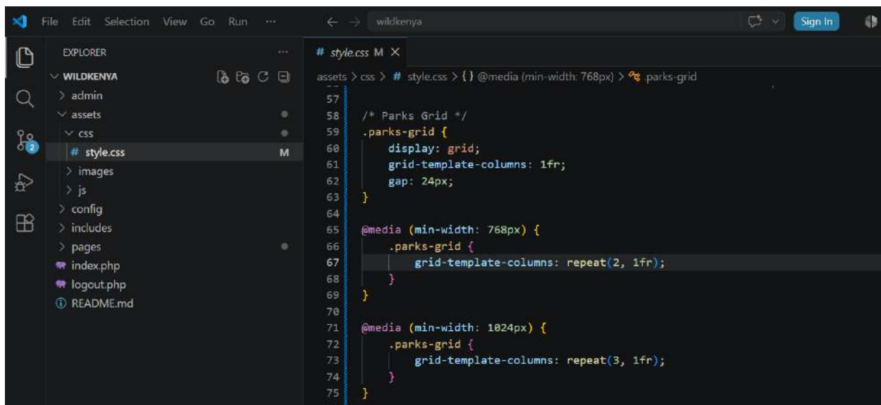
Fig 4- style.css showing CSS Grid media query breakpoints
