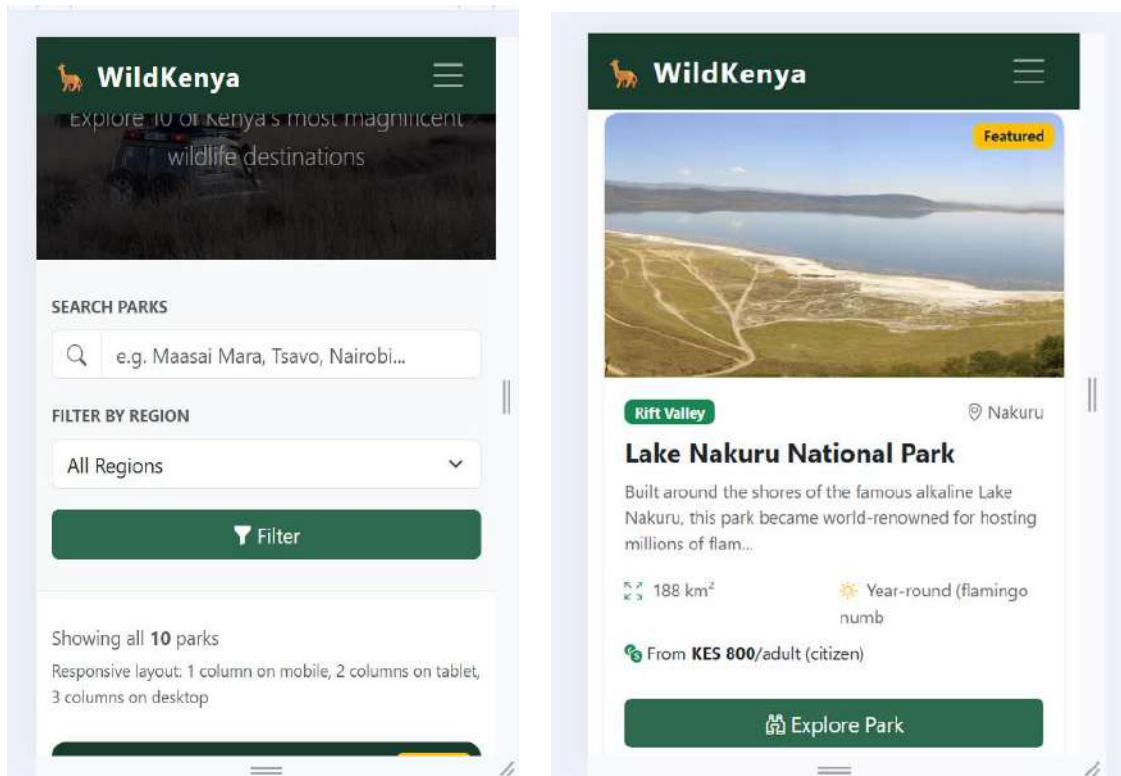
Fig 2- Parks page on mobile (375px) showing single column Mobile-First layout
