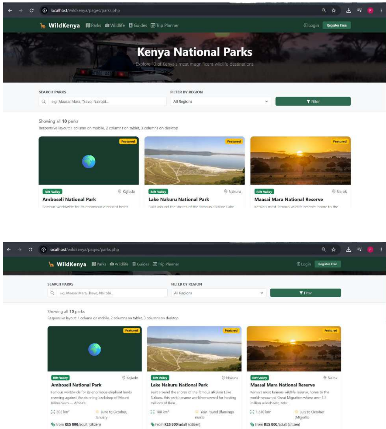
Fig 1- Parks page on desktop showing 3-column CSS Grid layout
